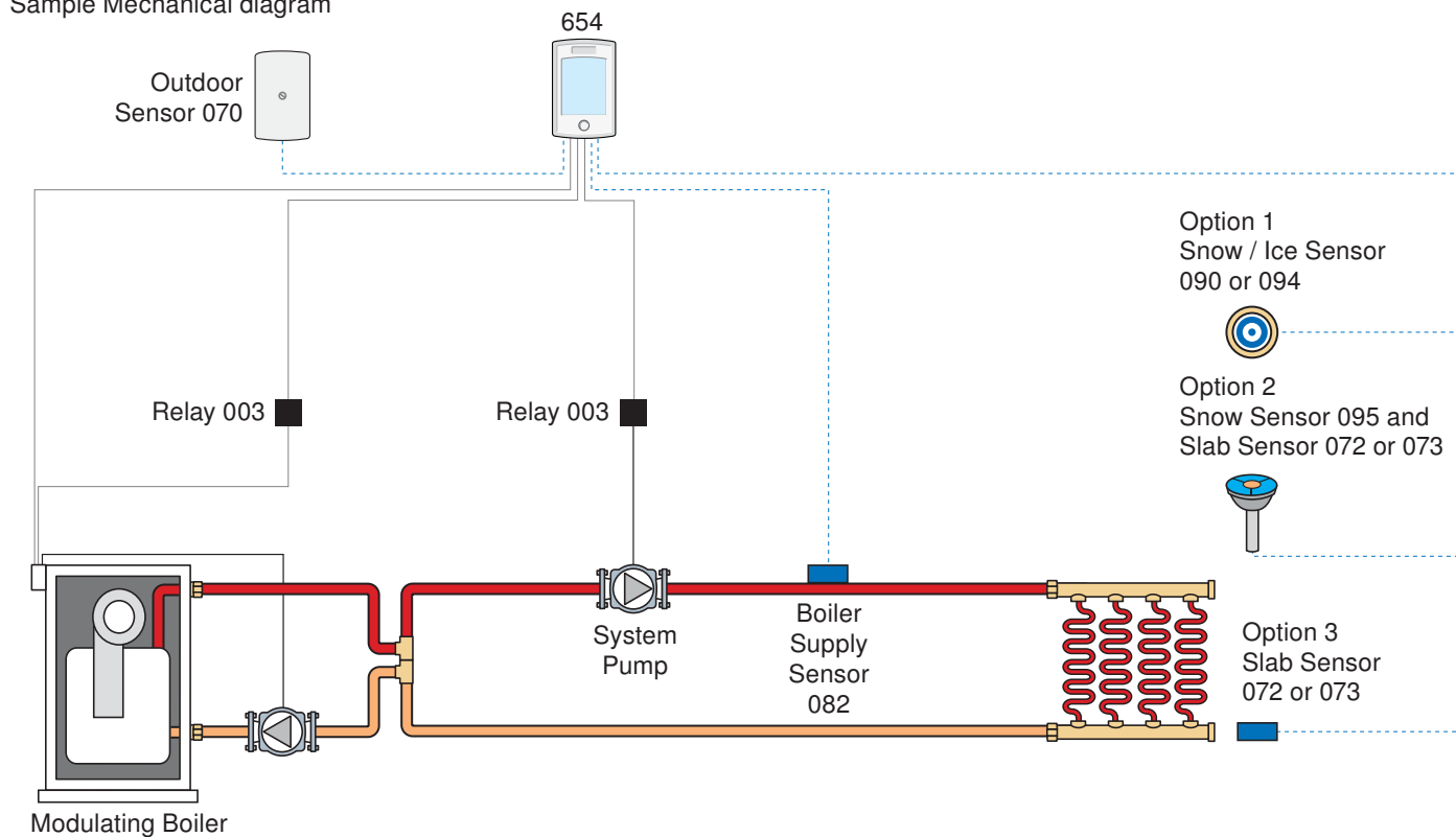
Sample Mechanical diagram
